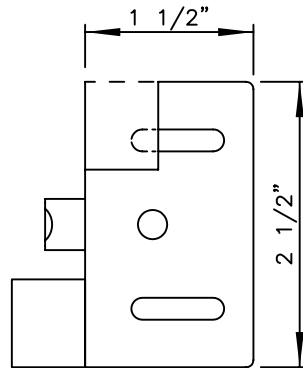
PLAN OF CAP SEAM CLIP
