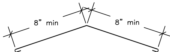
HIP / RIDGE
