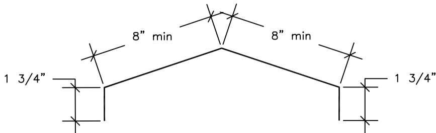
HIP / RIDGE (OPTIONAL)
