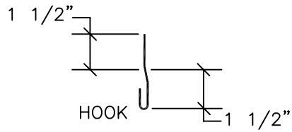
Offset Cleat
