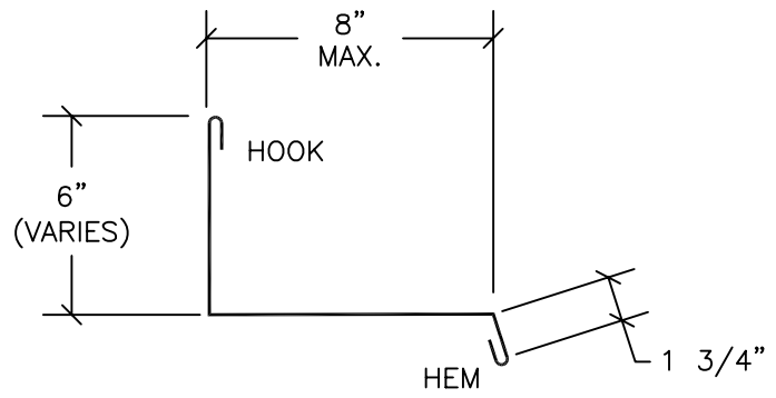
SIDEWALL
