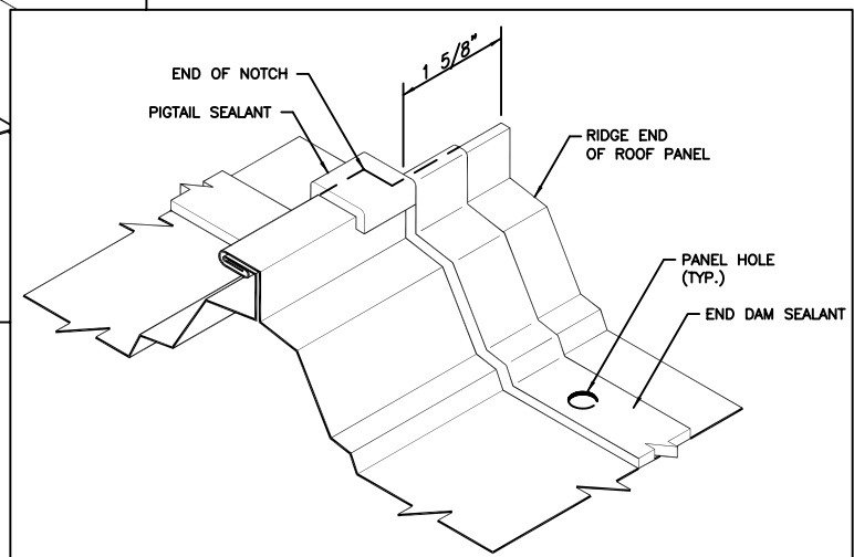
SEALANT DETAIL AT RIDGE
