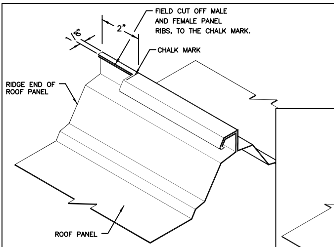
NOTCH FOR RIDGE CLOSURE
