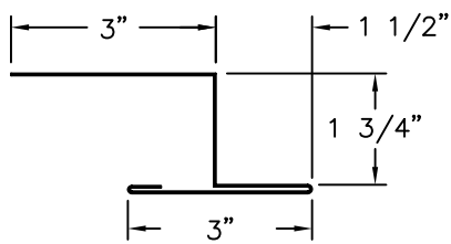
END SPLICE
