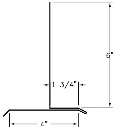
DOOR/WINDOW TRIM
