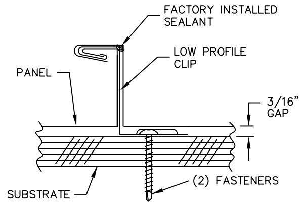
SEAMED LOW CLIP
