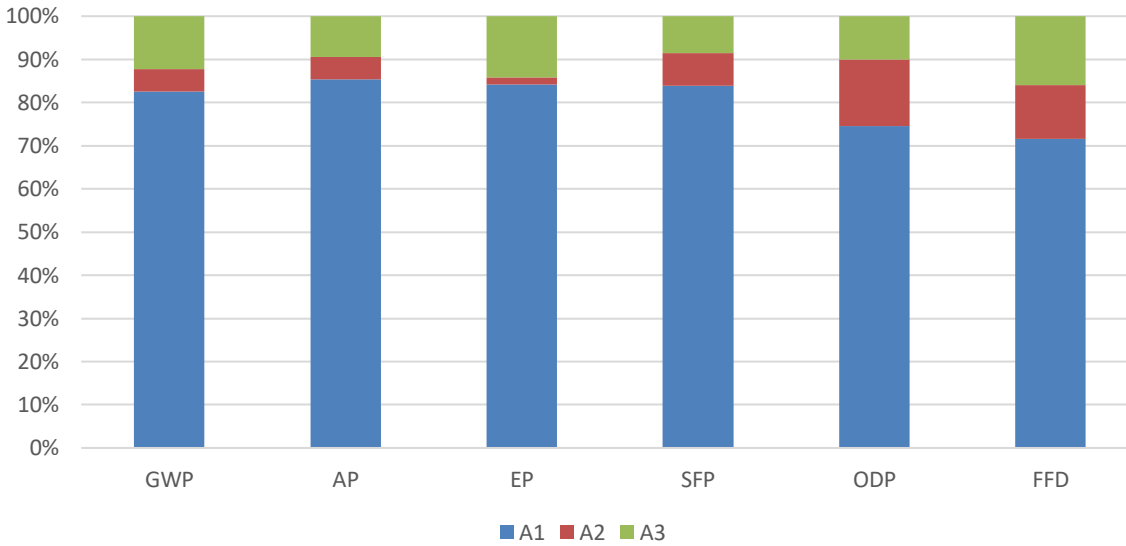
Figure 2. Contribution analysis for the AEP Span, manufactured from EAF Steel, using TRACI 2.1.
