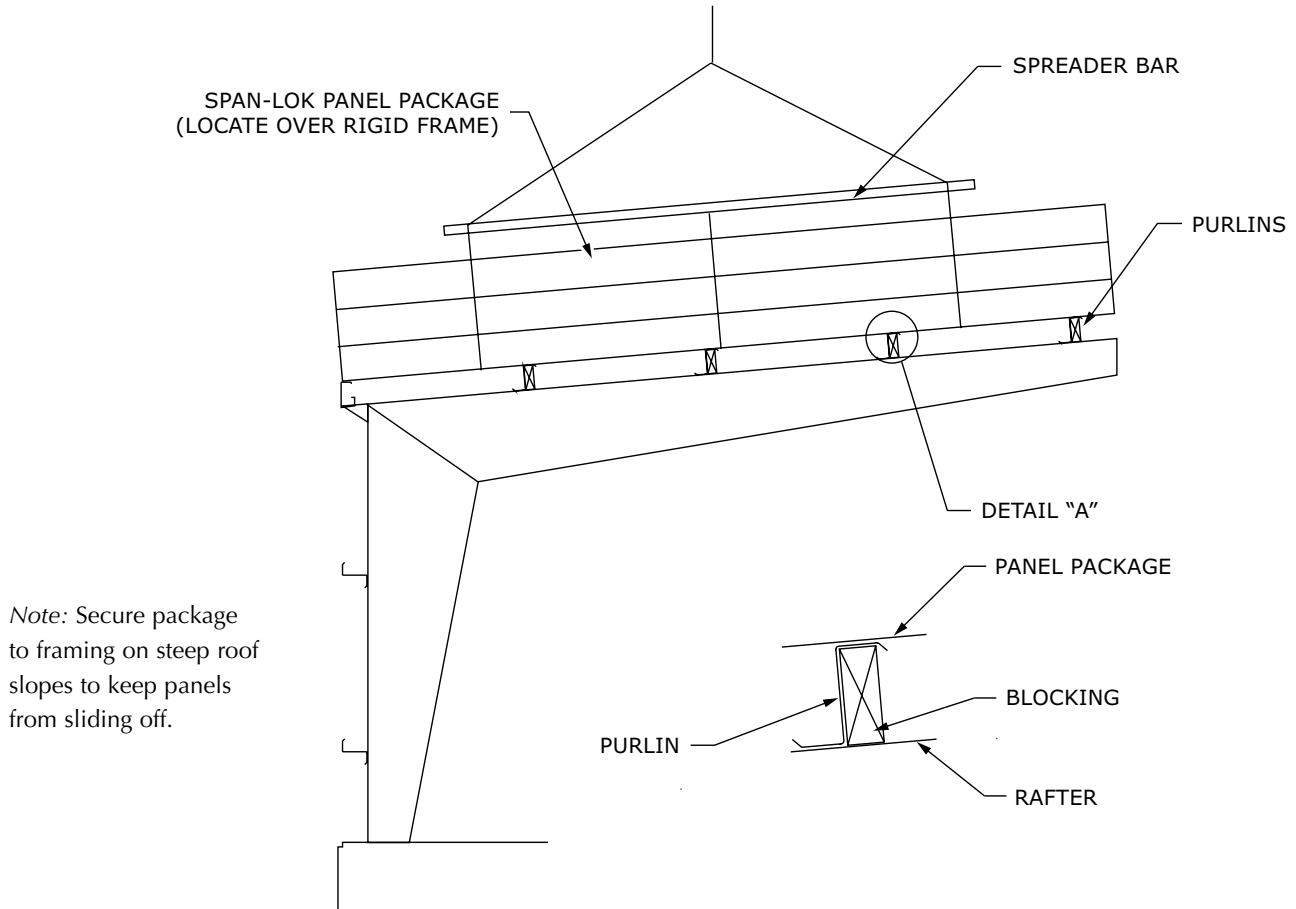
Detail "A"
