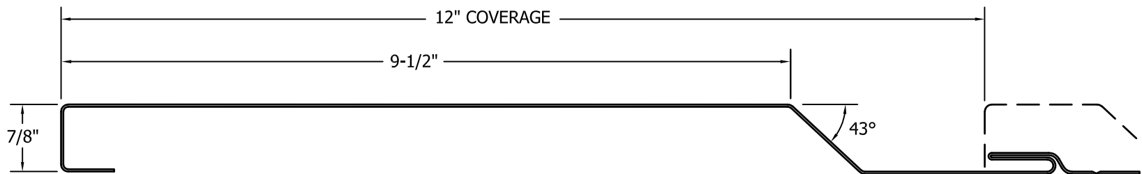
PC50-12d (DIRECT FASTENED)
