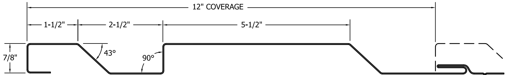
PC20-12d (DIRECT FASTENED)
