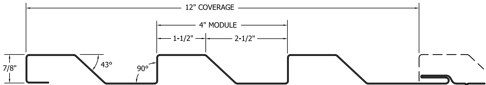
PC10-12d (DIRECT FASTENED)
