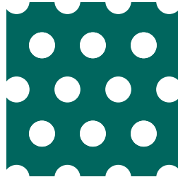
2 23.5% Open Area 0.191" Diameter 0.375" Spacing
