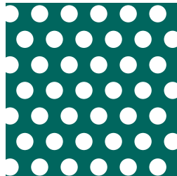
6 30.6% Open Area 0.127" Diameter 0.219" Spacing
