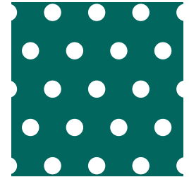
4 13.8% Open Area 0.127" Diameter 0.326" Spacing
