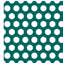
7 41.4% Open Area 0.127" Diameter 0.188" Spacing
