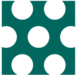
1 40.3% Open Area 0.375" Diameter 0.562" Spacing
