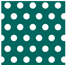
5 23.4% OPEN AREA 0.127" Diameter 0.25" Spacing
