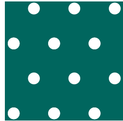
3 7.8% Open Area 0.127" Diameter 0.433" Spacing
