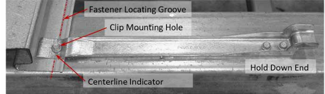
Fig. 2 Clip Installation
