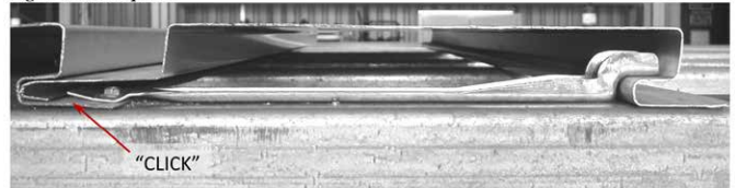
Fig. 4 Installed panel
