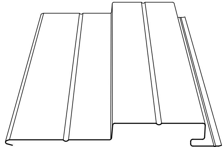
6 UP / 6 DOWN (SHOWN WITH RIBS)
