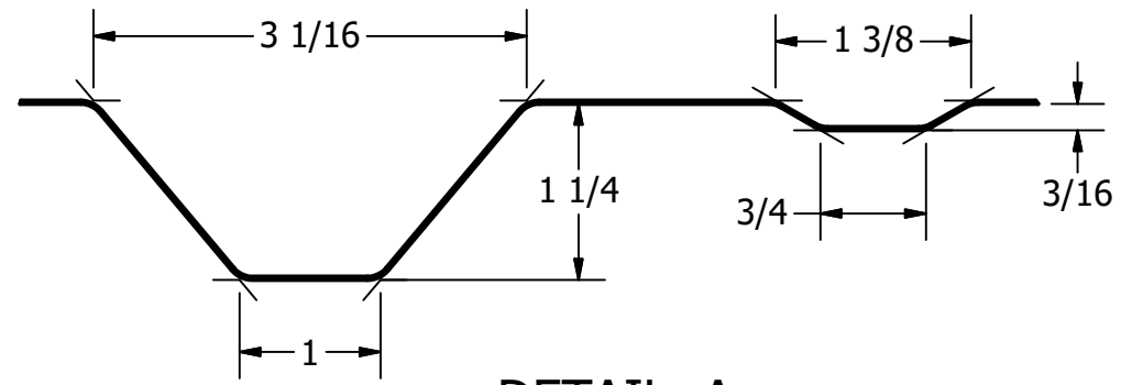
DETAIL A
