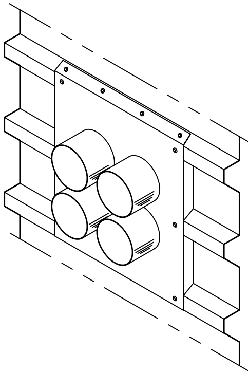
AC PIPING PENETRATION
