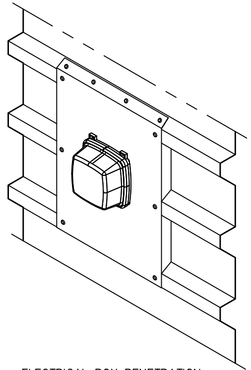
ELECTRICAL BOX PENETRATION
