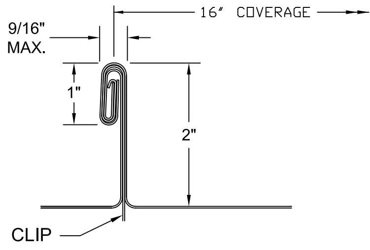
INSTALLED VIEW
